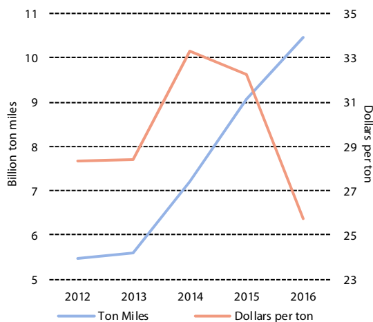
Diagram 34: Barge volumes and rates
