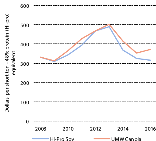
Diagram 30: Protein-adjusted prices for canola and soy meal
